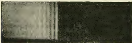
FIG. 10.—Fluting of magnesium.
